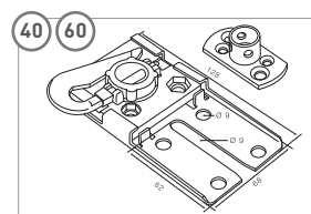
Abrolllager-Metall/PCV
