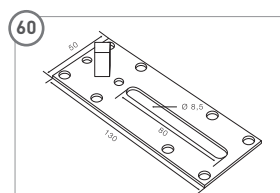
Lager Metall*
